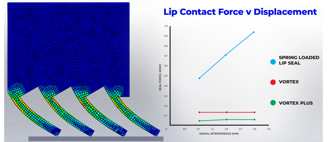
Unlike traditional lip seals, VORTEX maintains a constant seal force across a range of deflections
