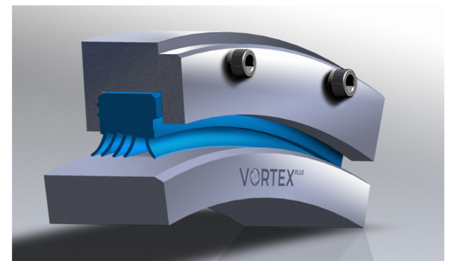
VORTEX and VORTEX PLUS in installed state. Note that the latter dust wiper still faces outward to prevent ingress
